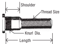
SERRATED BOLTS
