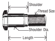
SHOULDER BOLTS
