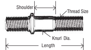
DOUBLE ENDED STUDS
